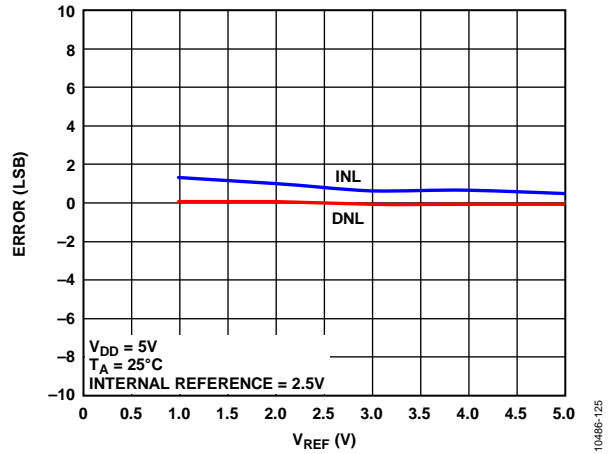
Figure 20. INL Error and DNL Error vs. V_{REF}
