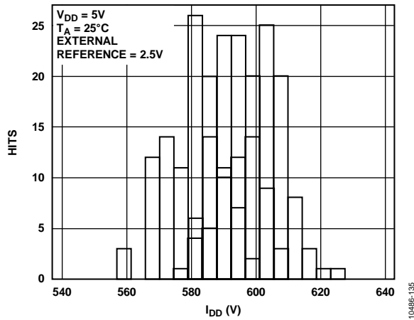
Figure 29. I_{DD} Histogram with External Reference, 5 V
