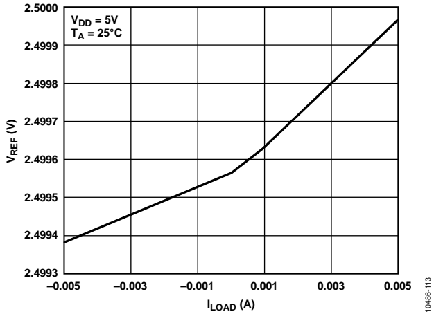
Figure 11. Internal Reference Voltage vs. Load Current
