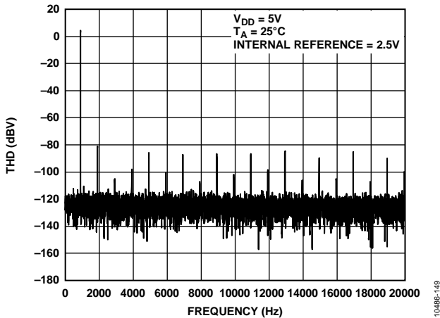
Figure 43. Total Harmonic Distortion @ 1 kHz
