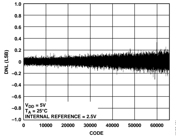
Figure 16. AD5696R DNL
