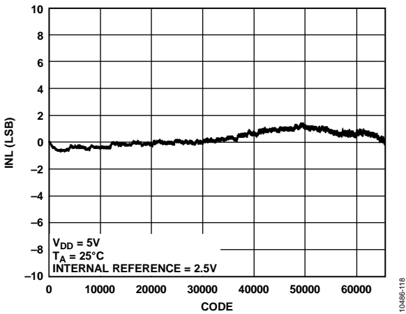
Figure 13. AD5696R INL
