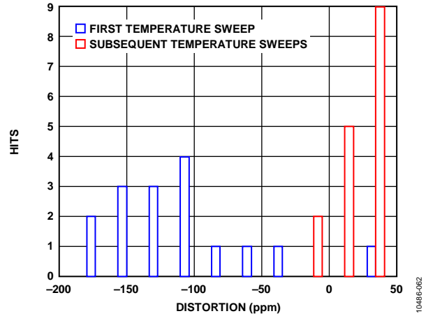
Figure 57. Thermal Hysteresis
