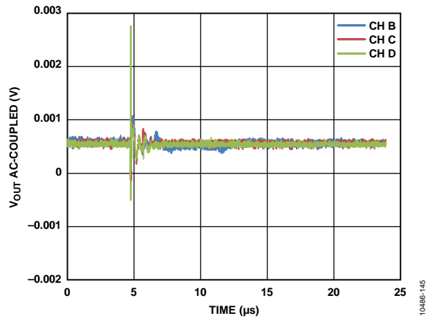
Figure 39. Analog Crosstalk, Channel A
