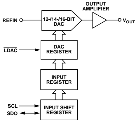
Figure 54. Simplified Diagram of Input Loading Circuitry for a Single DAC
