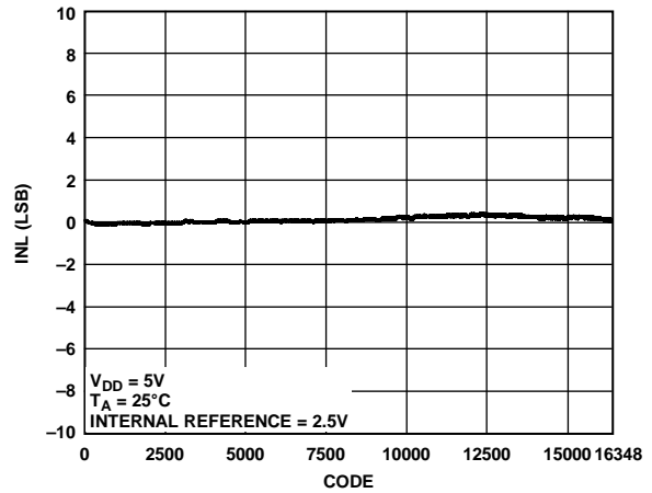
Figure 14. AD5695R INL
