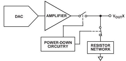
Figure 53. Output Stage During Power-Down
