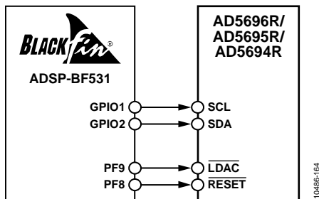
Figure 58. ADSP-BF531 Interface
