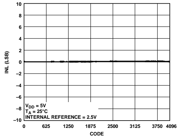
Figure 15. AD5694R INL
