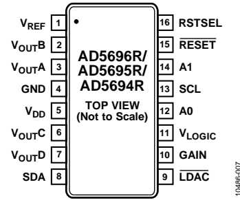
Figure 4. 16-Lead TSSOP Pin Configuration
