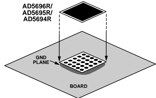
Figure 59. Paddle Connection to Board
