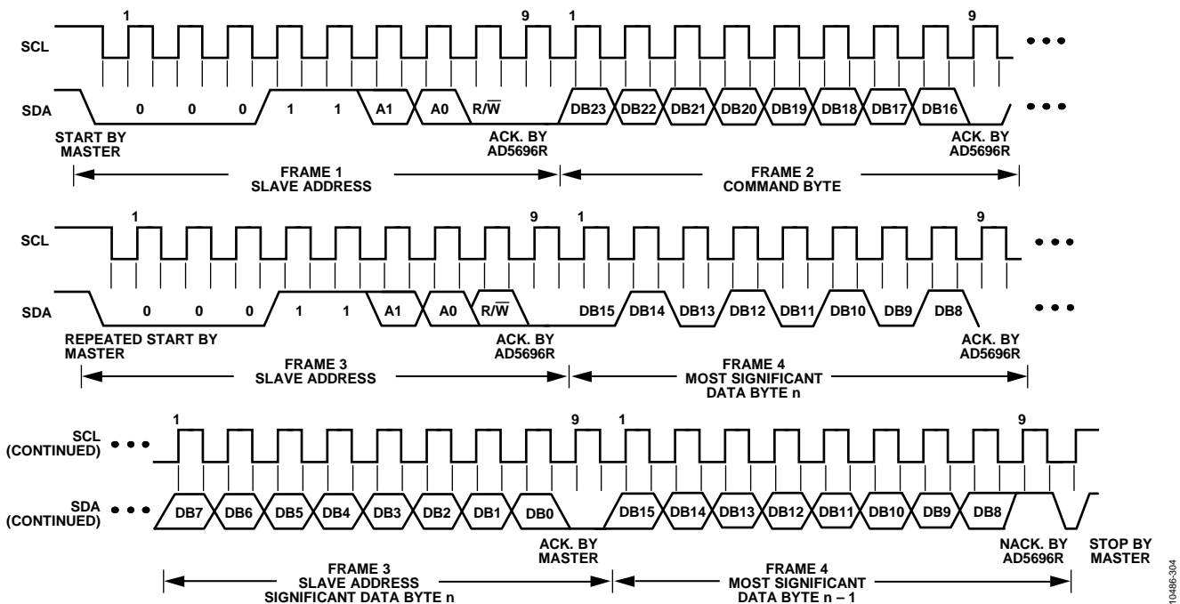
Figure 52. I 2 C Read Operation
