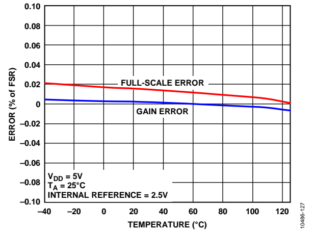
Figure 22. Gain Error and Full-Scale Error vs. Temperature
